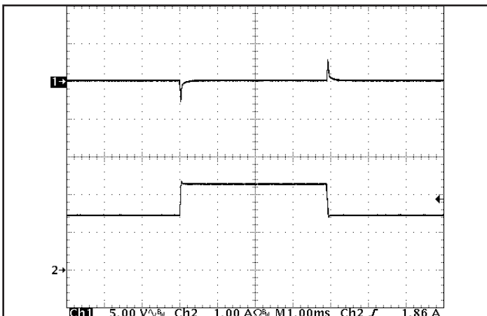
Figure 5: Output voltage response to step-change in load current (66% -100% -66% of I out (max); dI/dt = 0.02 A/μs). Load cap: 1 μF ceramic capacitor. Ch 1: V out (5 V/div), Ch 2: I out (1 A/div).
