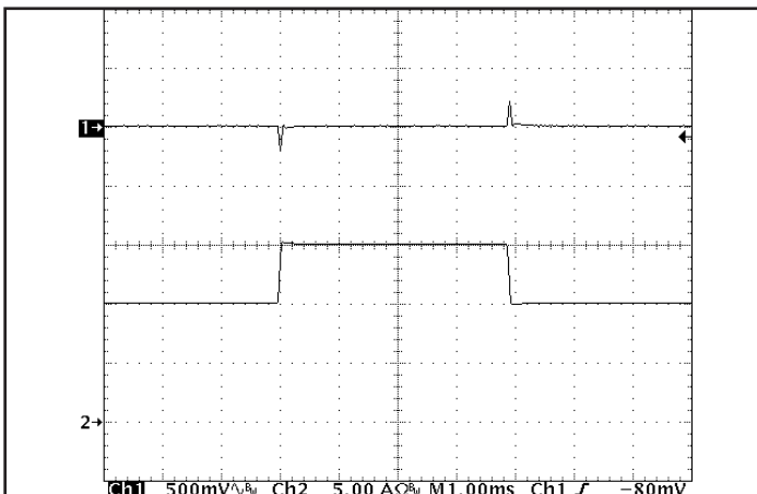
Figure 5: Output voltage response to step-change in load current (66% -100% -66% of Iout(max); dI/dt = 0.1 A/μs). Load cap: 1 μF ceramic and 15 μF tantalum capacitors. Ch 1: Vout (500 mV/div), Ch 2: Iout (5 A/div).
